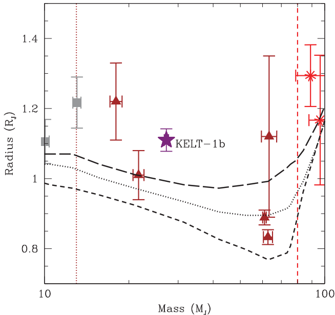
FIG. 18.— Radius versus mass for the known transiting companions to main-sequence stars with companion masses in the range 10–100 M_J that have measured radii. An estimate of the deuterium burning limit (Spiegel et al. 2011) is shown as the vertical dotted line, and the hydrogen burning limit is shown as the vertical dashed line. Brown dwarfs are shown as triangles, exoplanets as squares, and low-mass stars as asterisks. KELT-1b is shown as the large star. Predicted radii as a function of mass for isolated objects from the isochrones of Baraffe et al. (2003) are shown for an age of 5 Gyr (dashed), 1 Gyr (dotted), and 0.5 Gyr (long dashed); the true age of the KELT-1 system is almost certainly between 1–5 Gyr. Although stellar insolation is likely to increase the radii at fixed mass, Bouchy et al. (2011a) predict that the effect is small. KELT-1b therefore has an anomalously large radius.
